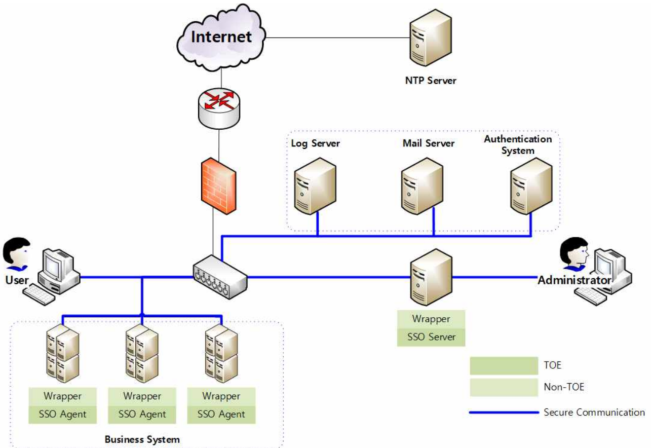
[Figure 2] TOE operational environment
